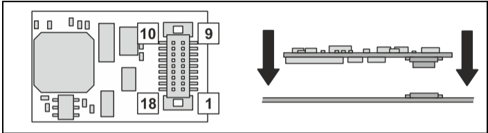
Abb. 1: SILVER+ Next18: 18-polige Schnittstelle NEM662 18-pole interface NEM662 18-pole Interface NEM662
